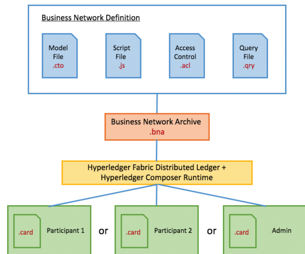
Figure 2—A framework to create a network via Hyperledger Composer.
