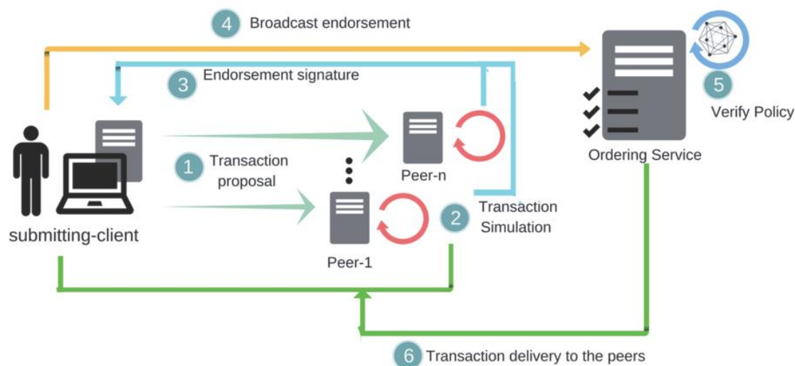
Figure 1: Outline of transaction flow in Hyperledger Fabric. It depicts a use case where: (1) A client node sends a transaction proposal to the endorsing nodes (for this example, all the peer nodes act as
